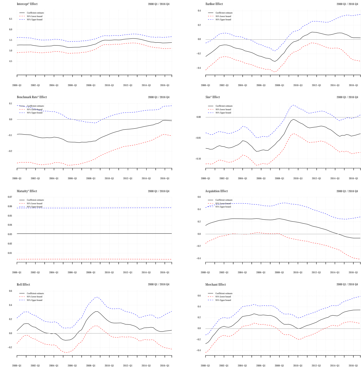
Figure 6: Infrastructure Project Debt Spread Factors – Time-Varying Factor Effects
